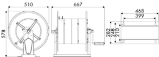
Abmessungen Modelle 75600/10, 75600/16, 75620/10, 75620/16, 75640/20, 75640/26, 75640/30
