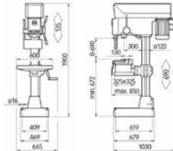
R32VS PGM
