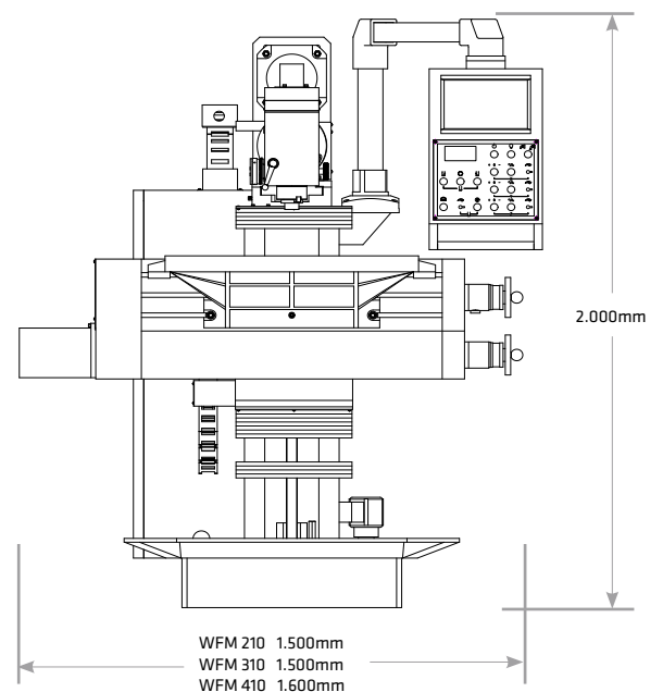
WFM 410 Servodrive
