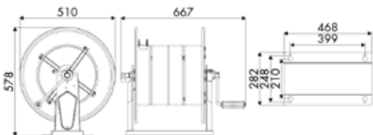
Abmessungen Modelle 75600/10, 75600/16, 75620/10, 75620/16, 75640/20, 75640/26, 75640/30
